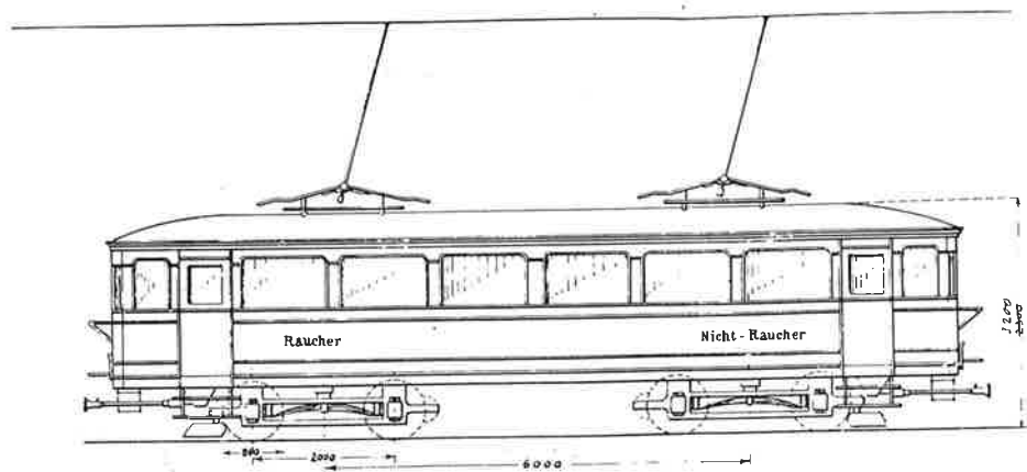
VIERACHSIGER MOTORWAGEN
